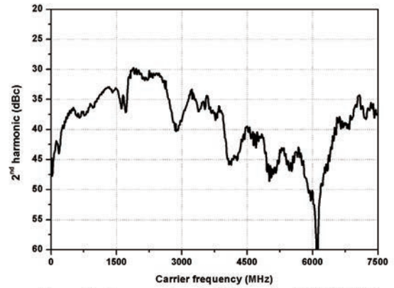
Measured tracking generator output 2 nd harmonic of DSA832/DSA875
